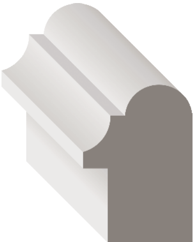
Stock Code 3652BBPOP (1521847) Dimensions 1 1/8" x 1 5/8" x RL FITS 3/4" CASING POP
