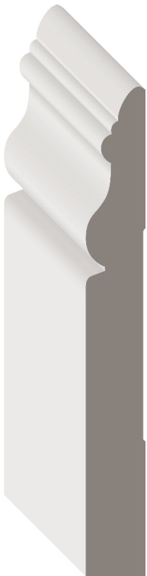
Stock Code 20160BM (1521486) Dimensions 5/8" x 5" x 16' MDF/UL
