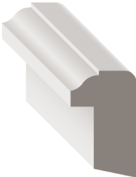
Stock Code 281LPRI (1521716) Dimensions 1 1/16" x 1 1/8" x 16' FITS 1 1/16" TO 3/4" CASING PRI
