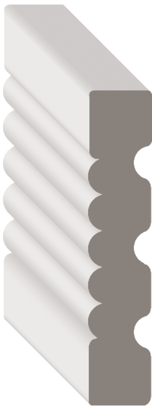
Stock Code Dimensions 194P \frac{5}{8}" \times 3\frac{1}{4}" \times 16' (1521468) PFJ
