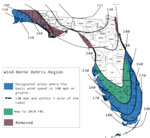
Figure 1609A Wind-Borne Debris Region, Category II and III Buildings and Structures except health care facilities
