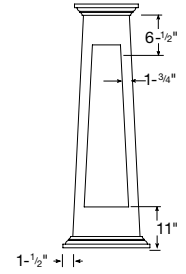
Recess is 1/2" deep and corners are 1/4" rounded.
